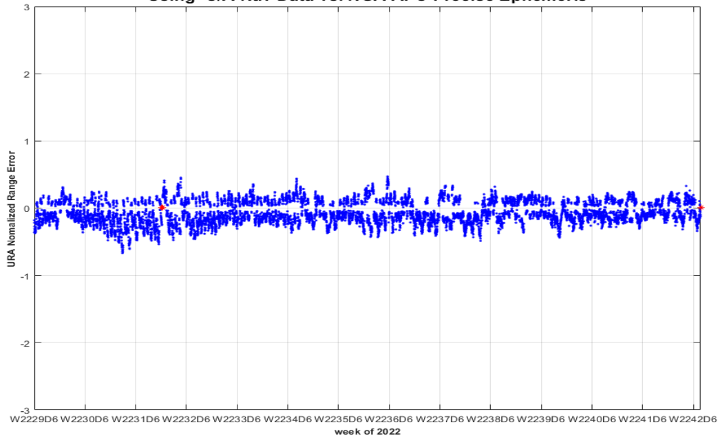
PRN-24 SVN-65 URA Normalized Range Error 10/01/2022 to 12/31/2022 (max in footprint) Using C/A Nav Data vs. NGA APC Precise Ephemeris
