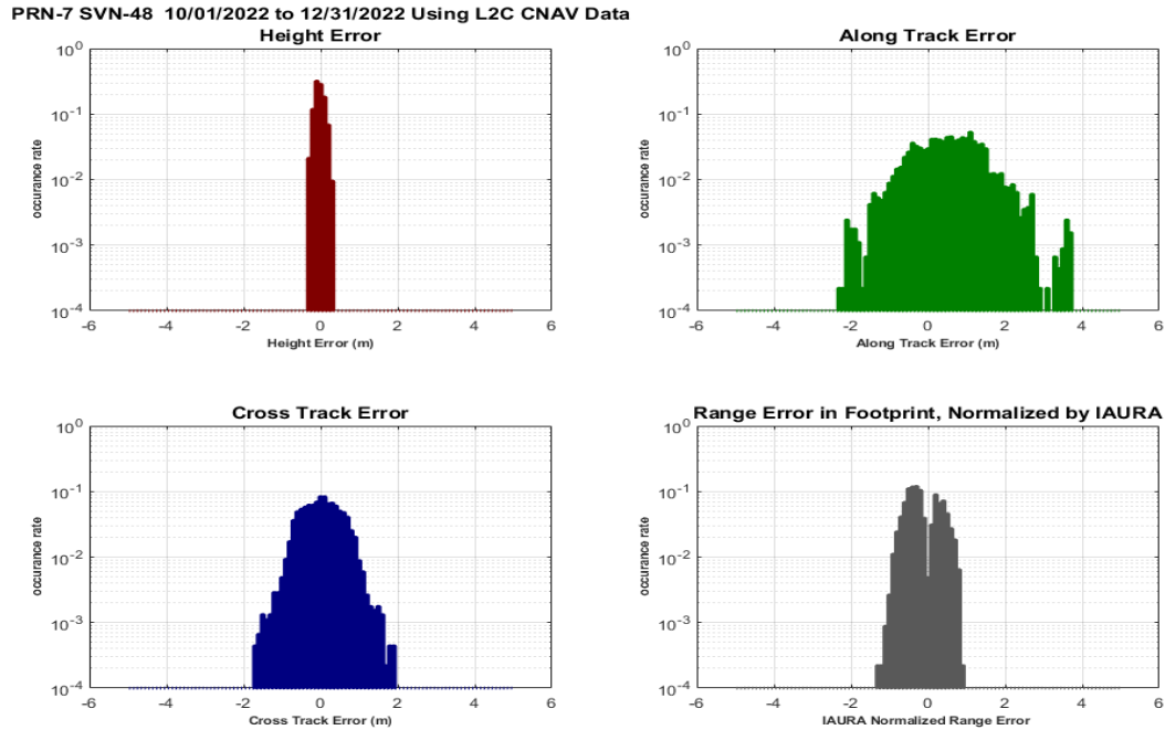
Figure 10-91 Histograms of H, A, C, and Range Error PRN7 (SVN48) Using L2C CNAV Data
