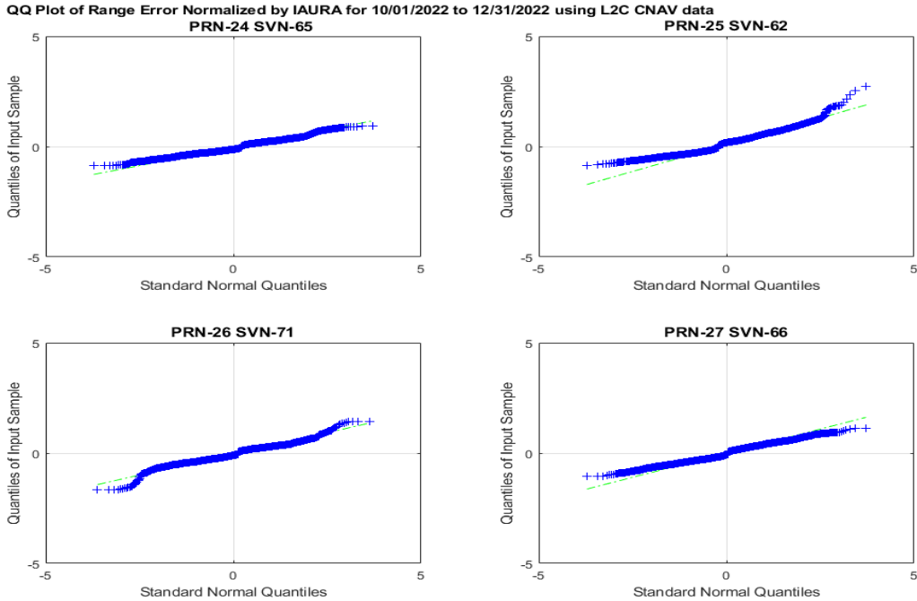
Figure 10-77 QQ Plots of Range Error PRN 24, 25, 26, and 27 Using L2C CNAV Data
