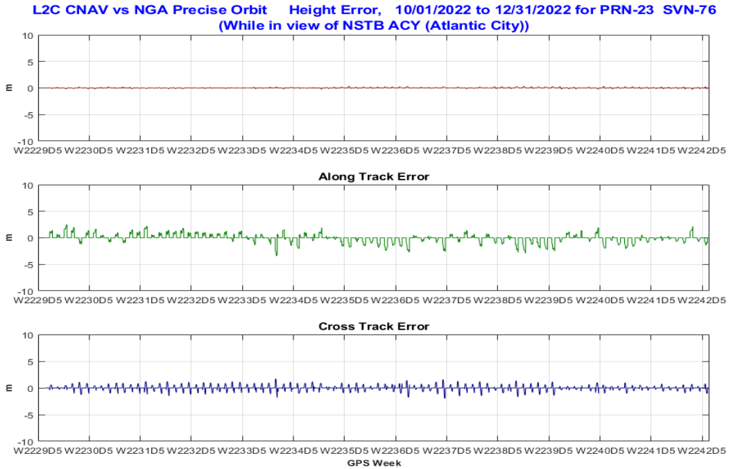
Figure 10-47 Orbit Error PRN23 (SVN76) Using L2C CNAV Data
