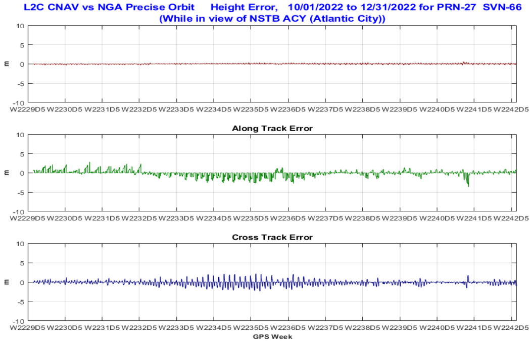
Figure 10-55 Orbit Error PRN27 (SVN66) Using L2C CNAV Data
