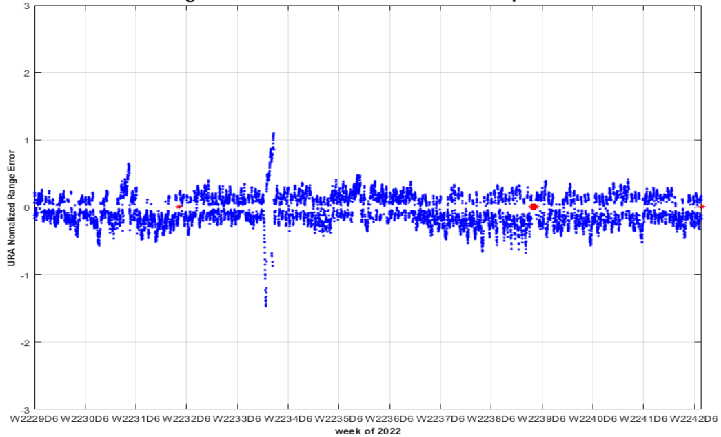
PRN-26 SVN-71 URA Normalized Range Error 10/01/2022 to 12/31/2022 (max in footprint) Using C/A Nav Data vs. NGA APC Precise Ephemeris
