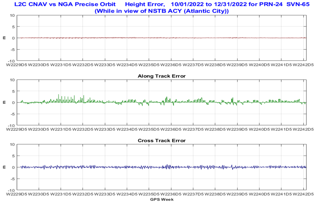
Figure 10-49 Orbit Error PRN24 (SVN65) Using L2C CNAV Data
