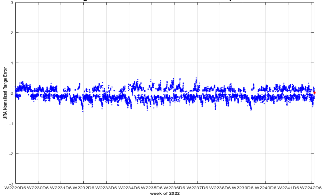
PRN-11 SVN-78 URA Normalized Range Error 10/01/2022 to 12/31/2022 (max in footprint) Using C/A Nav Data vs. NGA APC Precise Ephemeris
