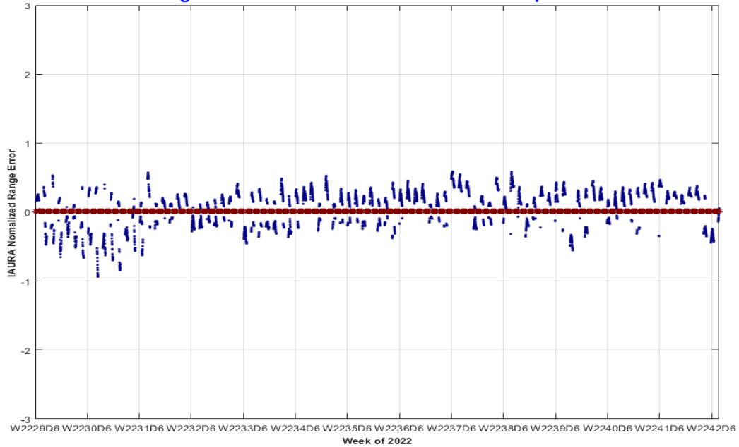
PRN-14 SVN-77 IAURA Normalized Range Error 10/01/2022 to 12/31/2022 (max in footprint) Using L2C CNAV Data vs. NGA APC Precise Ephemeris
