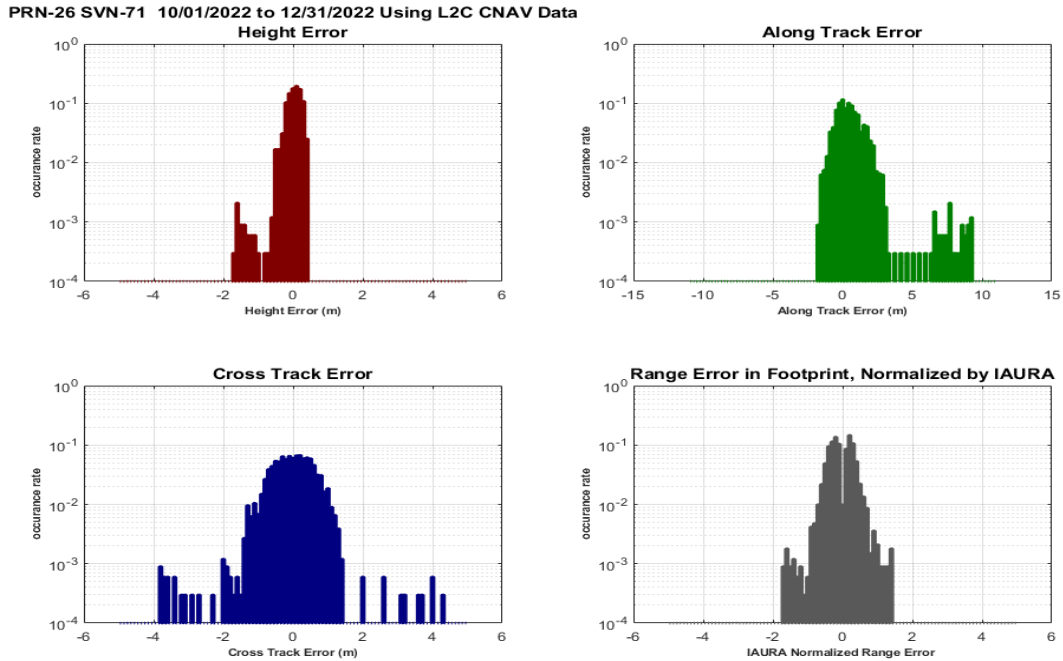
Figure 10-123 Histograms of H, A, C, and Range Error PRN26 (SVN71) Using L2C CNAV Data
