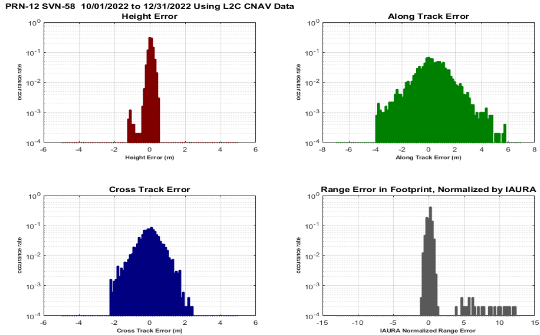
Figure 10-101 Histograms of H, A, C, and Range Error PRN12 (SVN58) Using L2C CNAV Data
