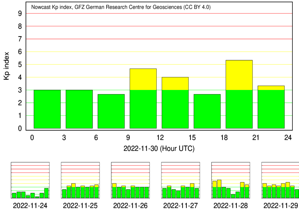
Figure 6-2 K-Index for November 30, 2022
