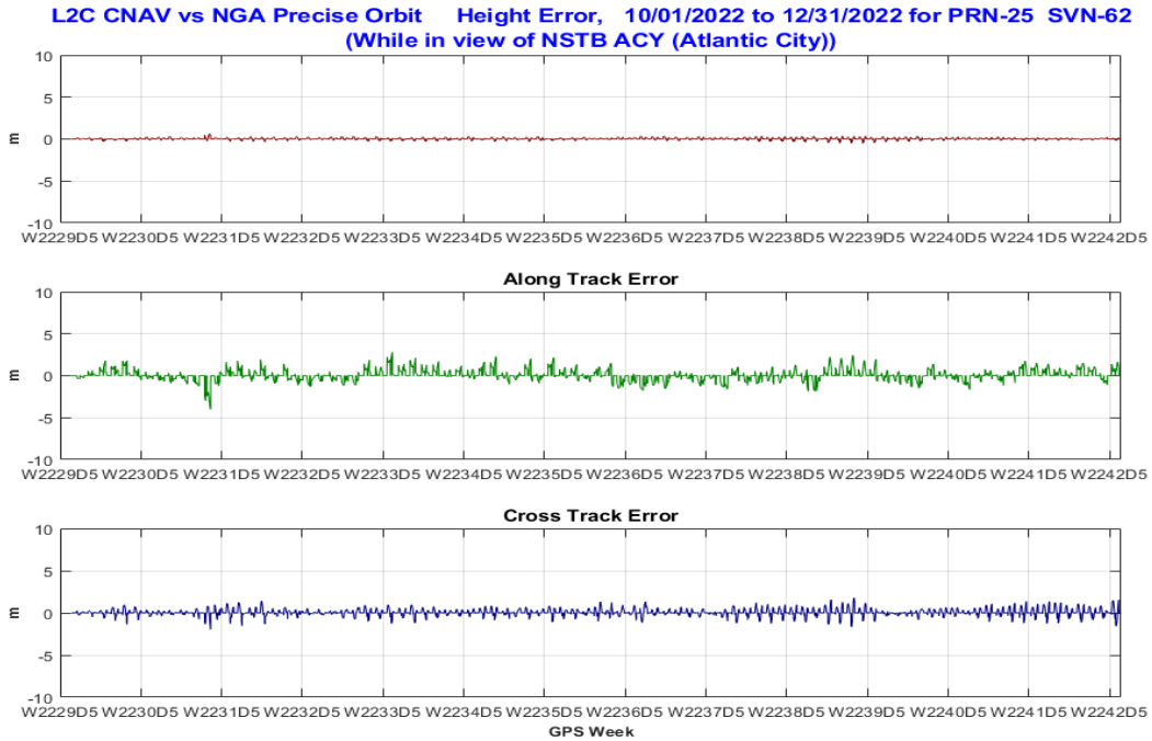
Figure 10-51 Orbit Error PRN25 (SVN62) Using L2C CNAV Data
