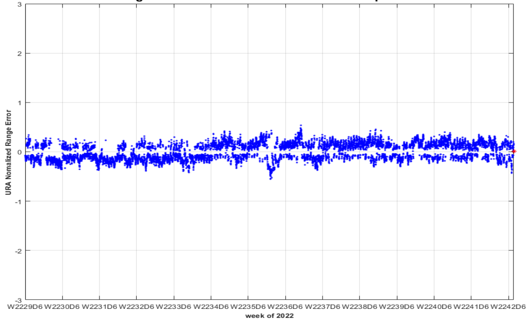
PRN-18 SVN-75 URA Normalized Range Error 10/01/2022 to 12/31/2022 (max in footprint) Using C/A Nav Data vs. NGA APC Precise Ephemeris
