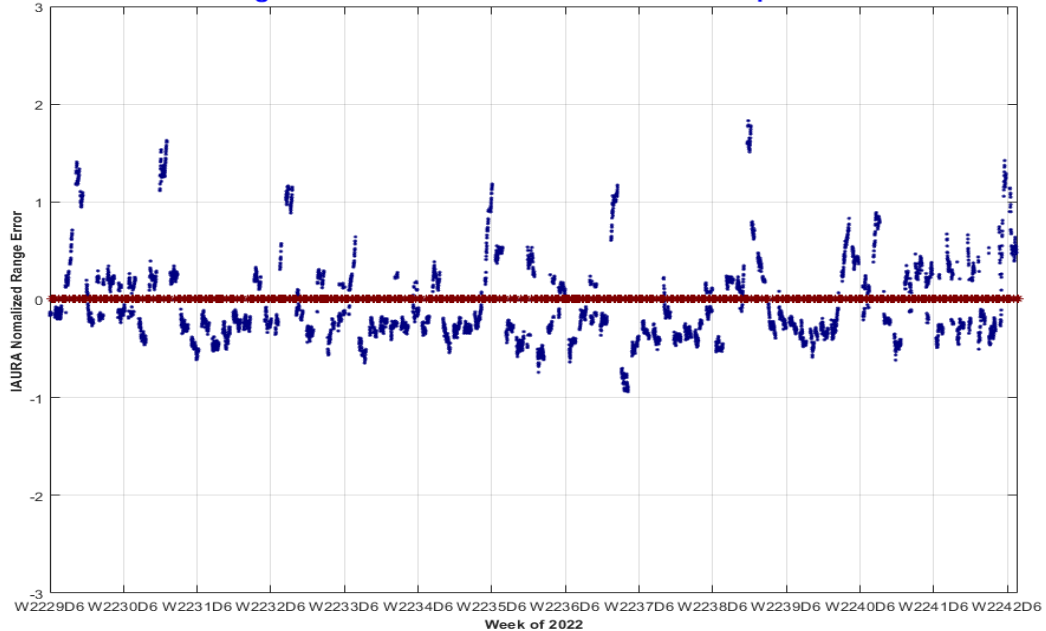
PRN-29 SVN-57 IAURA Normalized Range Error 10/01/2022 to 12/31/2022 (max in footprint) Using L2C CNAV Data vs. NGA APC Precise Ephemeris
