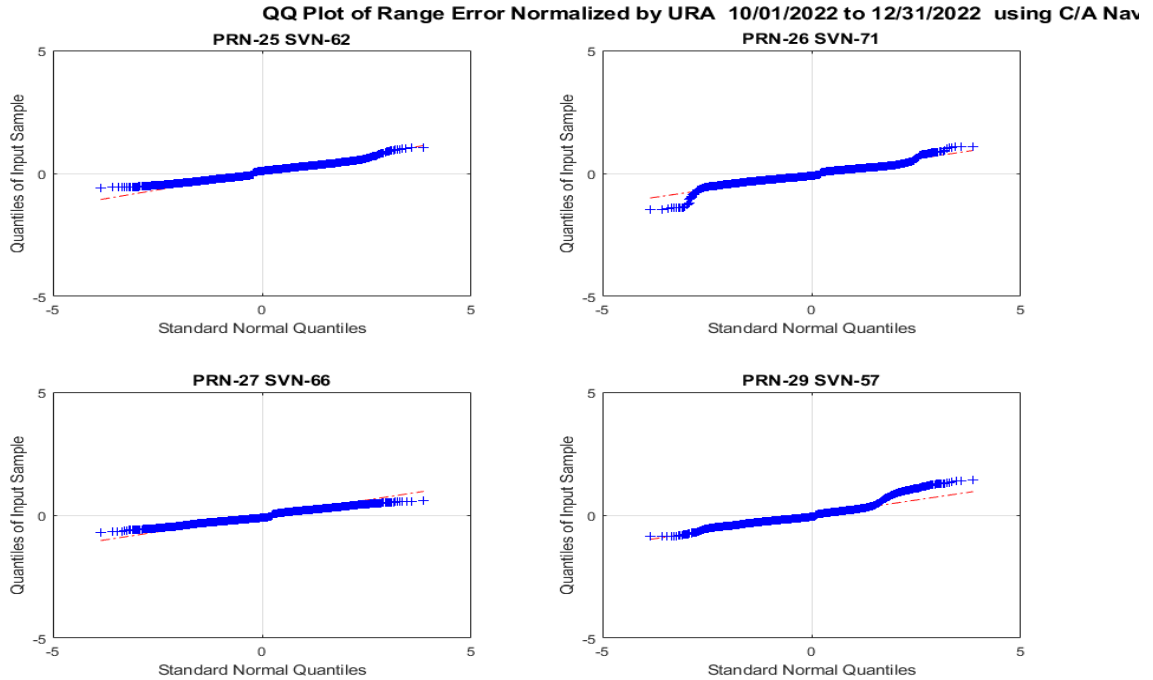
Figure 10-71 QQ Plots of Range Error PRNs 25 to 29 Using C/A Nav Data
