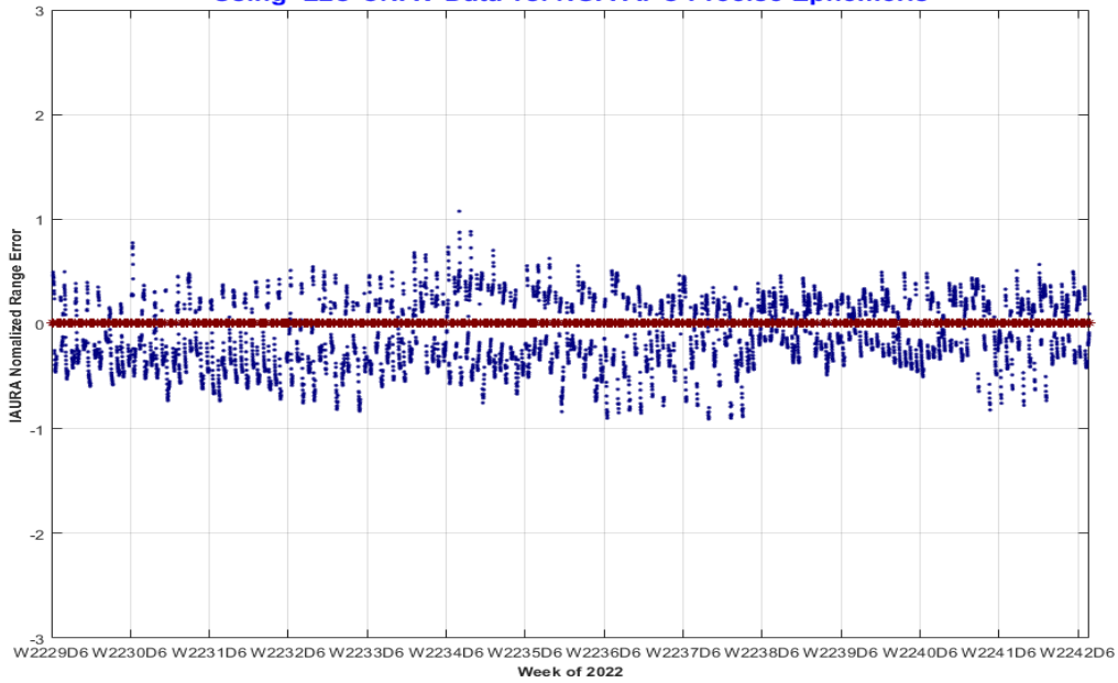
PRN-1 SVN-63 IAURA Normalized Range Error 10/01/2022 to 12/31/2022 (max in footprint) Using L2C CNAV Data vs. NGA APC Precise Ephemeris
