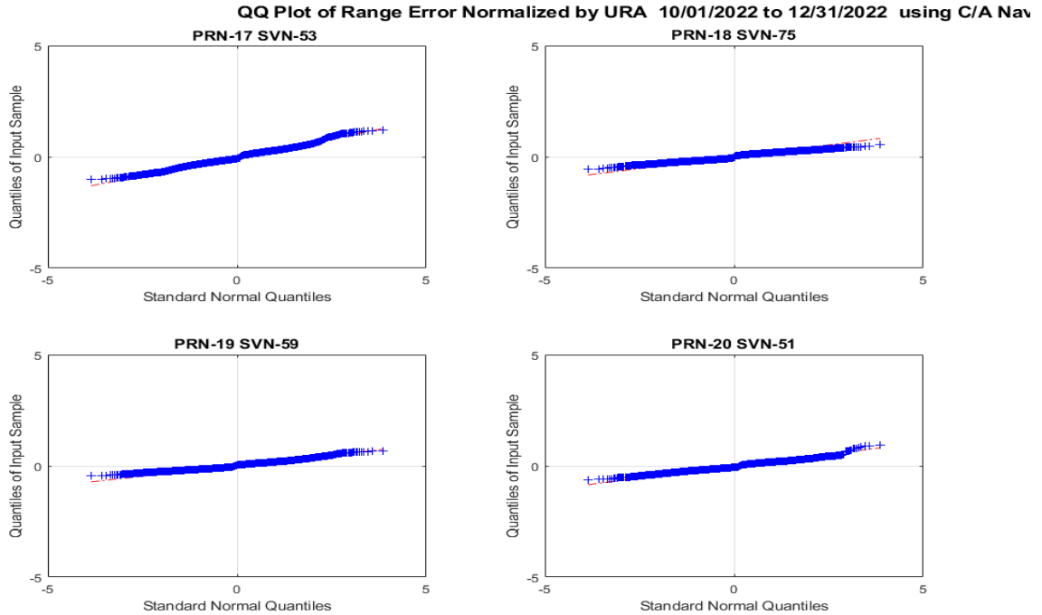
Figure 10-69 QQ Plots of Range Error PRNs 17 to 20 Using C/A Nav Data
