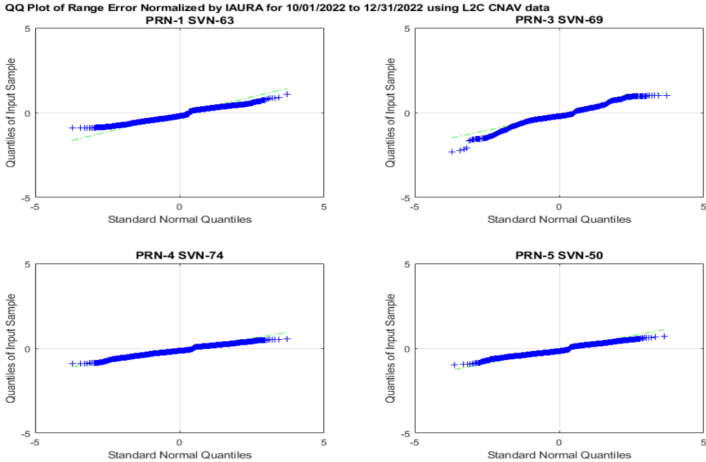
Figure 10-73 QQ Plots of Range Error PRNs 1, 3, 4, and 5 Using L2C CNAV Data
