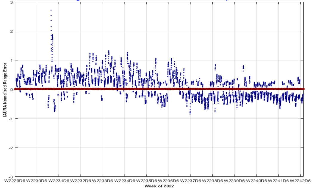
PRN-25 SVN-62 IAURA Normalized Range Error 10/01/2022 to 12/31/2022 (max in footprint) Using L2C CNAV Data vs. NGA APC Precise Ephemeris
