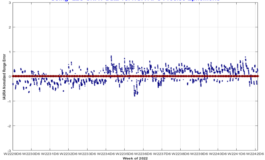
PRN-18 SVN-75 IAURA Normalized Range Error 10/01/2022 to 12/31/2022 (max in footprint) Using L2C CNAV Data vs. NGA APC Precise Ephemeris
