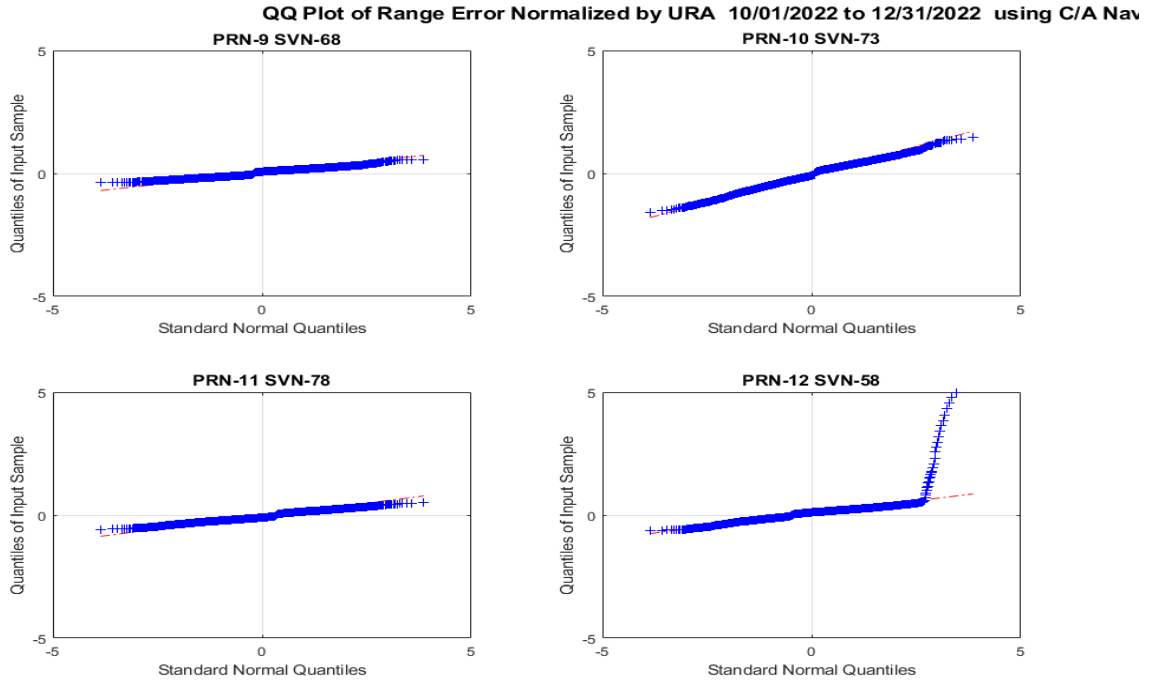
Figure 10-67 QQ Plots of Range Error PRNs 9 to 12 Using C/A Nav Data
