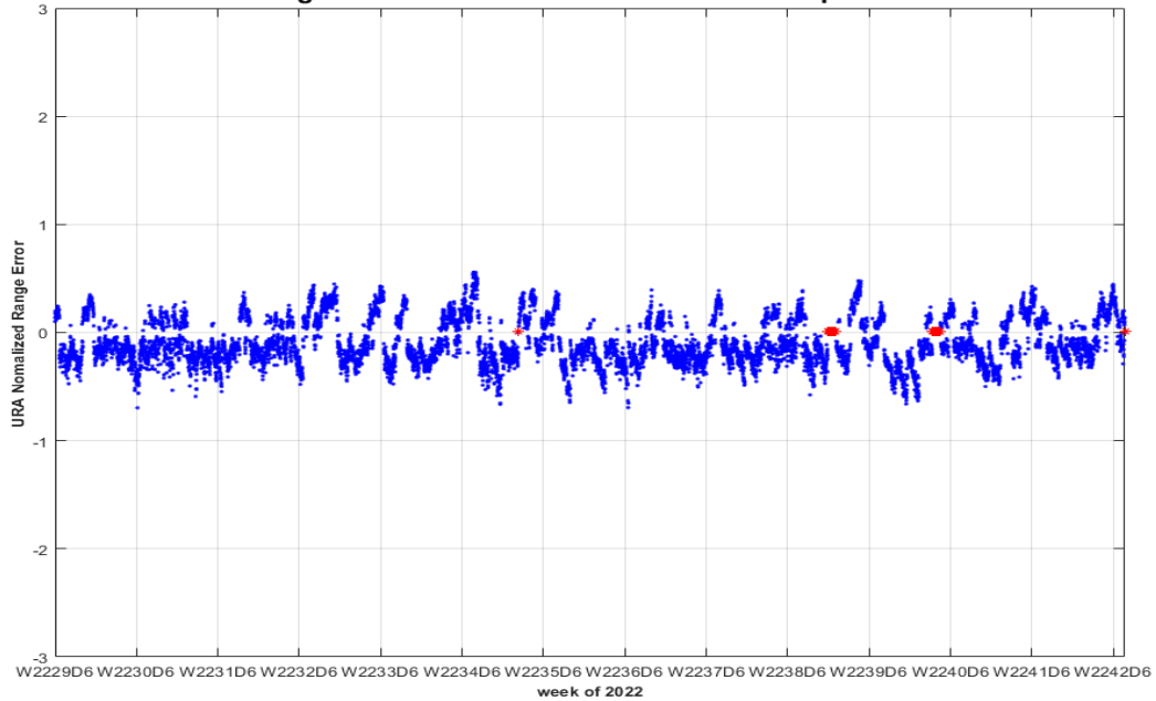
PRN-31 SVN-52 URA Normalized Range Error 10/01/2022 to 12/31/2022 (max in footprint) Using C/A Nav Data vs. NGA APC Precise Ephemeris
