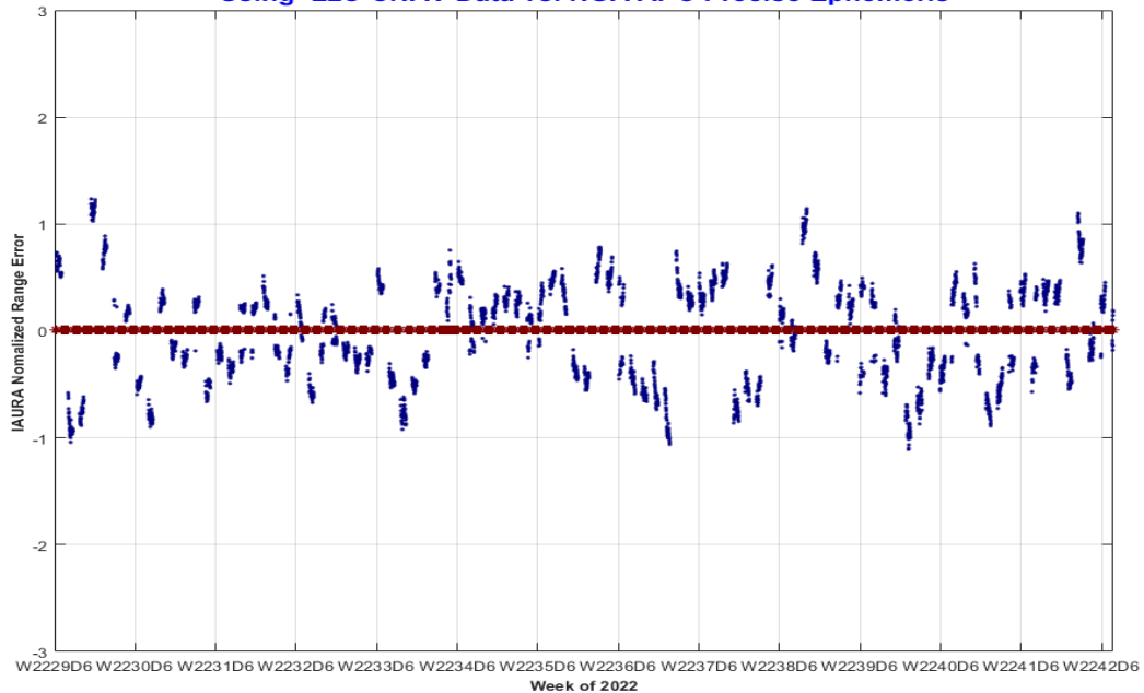
PRN-17 SVN-53 IAURA Normalized Range Error 10/01/2022 to 12/31/2022 (max in footprint) Using L2C CNAV Data vs. NGA APC Precise Ephemeris
