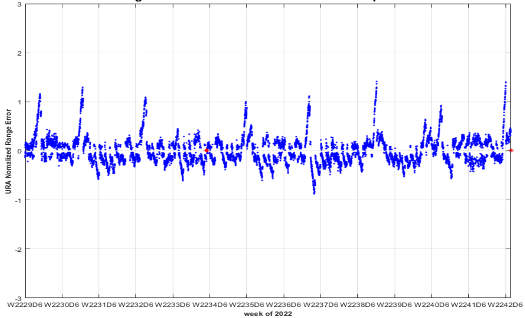
PRN-29 SVN-57 URA Normalized Range Error 10/01/2022 to 12/31/2022 (max in footprint) Using C/A Nav Data vs. NGA APC Precise Ephemeris
