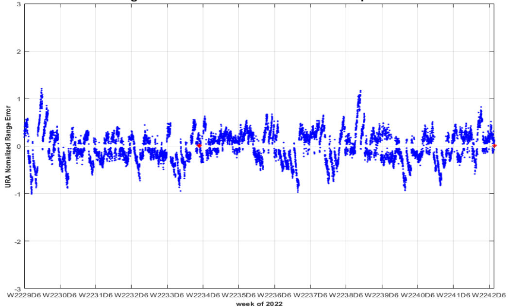
PRN-17 SVN-53 URA Normalized Range Error 10/01/2022 to 12/31/2022 (max in footprint) Using C/A Nav Data vs. NGA APC Precise Ephemeris
