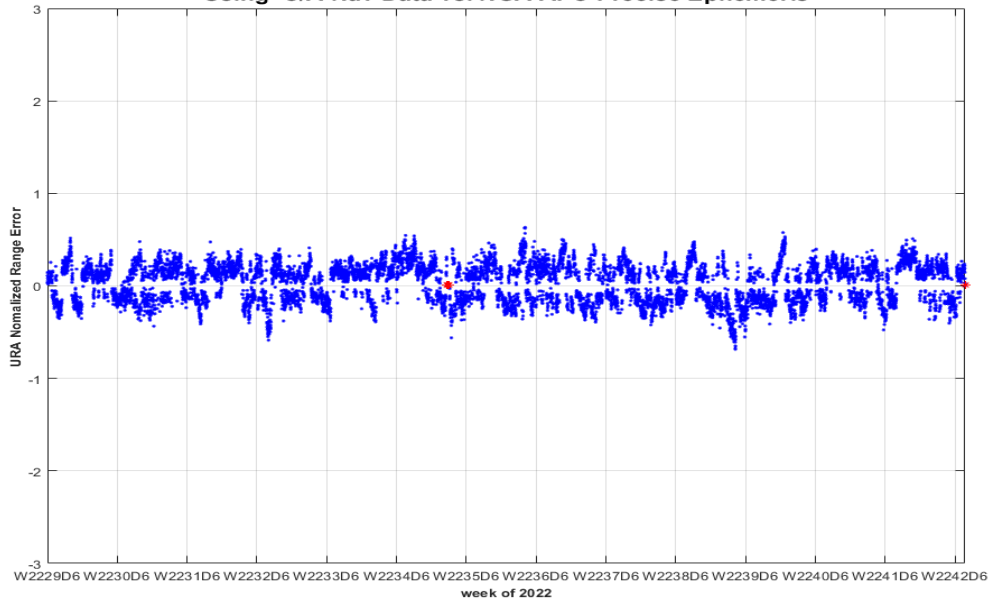
PRN-2 SVN-61 URA Normalized Range Error 10/01/2022 to 12/31/2022 (max in footprint) Using C/A Nav Data vs. NGA APC Precise Ephemeris
