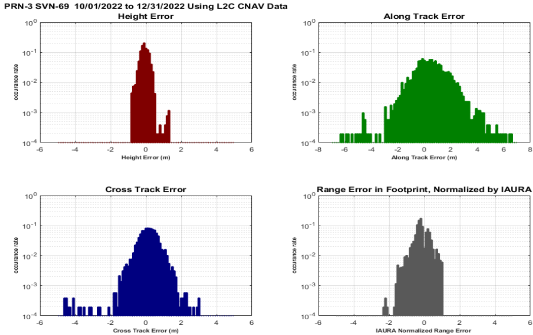
Figure 10-83 Histograms of H, A, C, and Range Error PRN3 (SVN69) Using L2C CNAV Data
