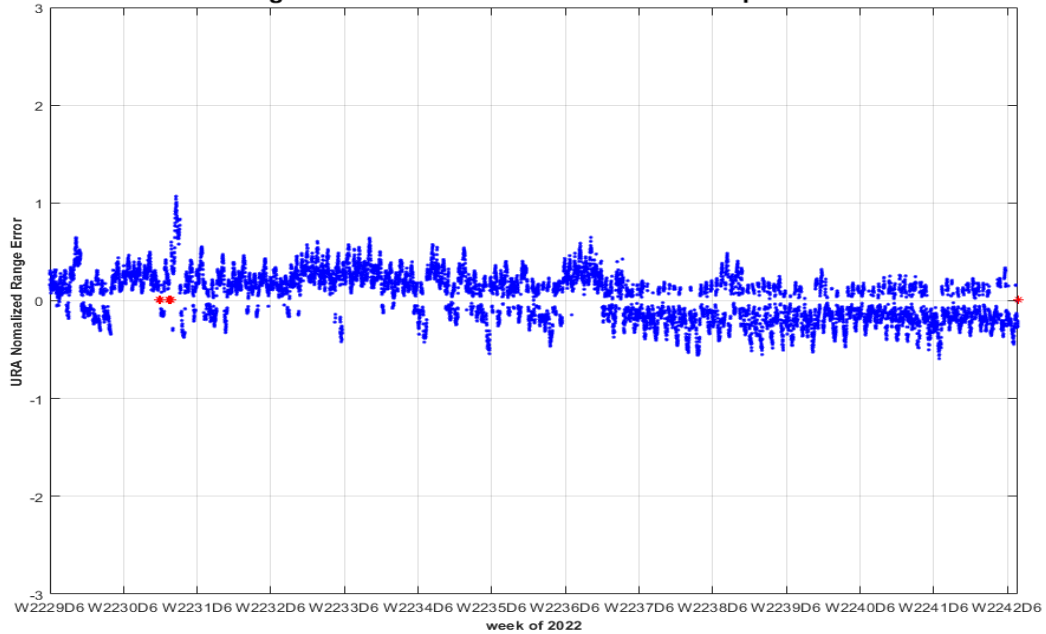
PRN-25 SVN-62 URA Normalized Range Error 10/01/2022 to 12/31/2022 (max in footprint) Using C/A Nav Data vs. NGA APC Precise Ephemeris
