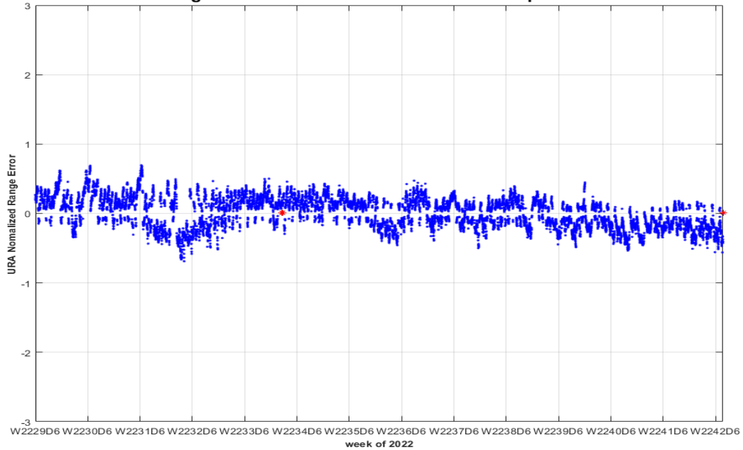
PRN-30 SVN-64 URA Normalized Range Error 10/01/2022 to 12/31/2022 (max in footprint) Using C/A Nav Data vs. NGA APC Precise Ephemeris
