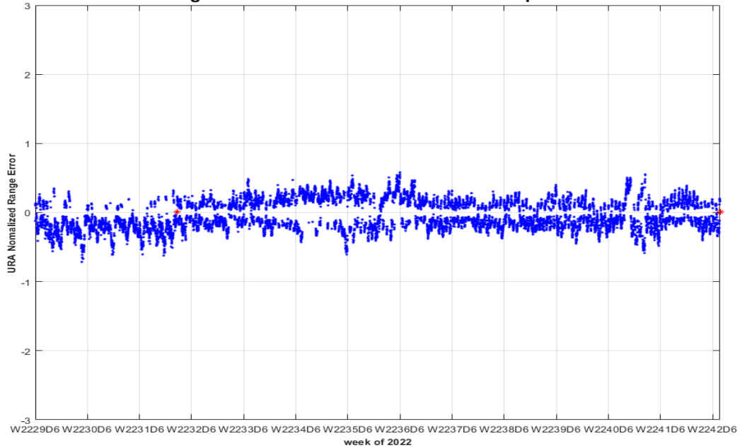
PRN-27 SVN-66 URA Normalized Range Error 10/01/2022 to 12/31/2022 (max in footprint) Using C/A Nav Data vs. NGA APC Precise Ephemeris
