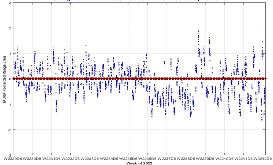
PRN-10 SVN-73 IAURA Normalized Range Error 10/01/2022 to 12/31/2022 (max in footprint) Using L2C CNAV Data vs. NGA APC Precise Ephemeris
