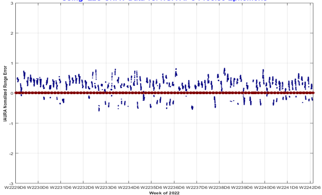
PRN-23 SVN-76 IAURA Normalized Range Error 10/01/2022 to 12/31/2022 (max in footprint) Using L2C CNAV Data vs. NGA APC Precise Ephemeris
