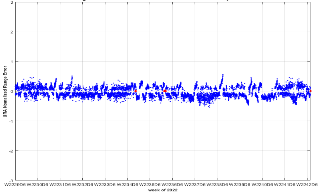
PRN-15 SVN-55 URA Normalized Range Error 10/01/2022 to 12/31/2022 (max in footprint) Using C/A Nav Data vs. NGA APC Precise Ephemeris
