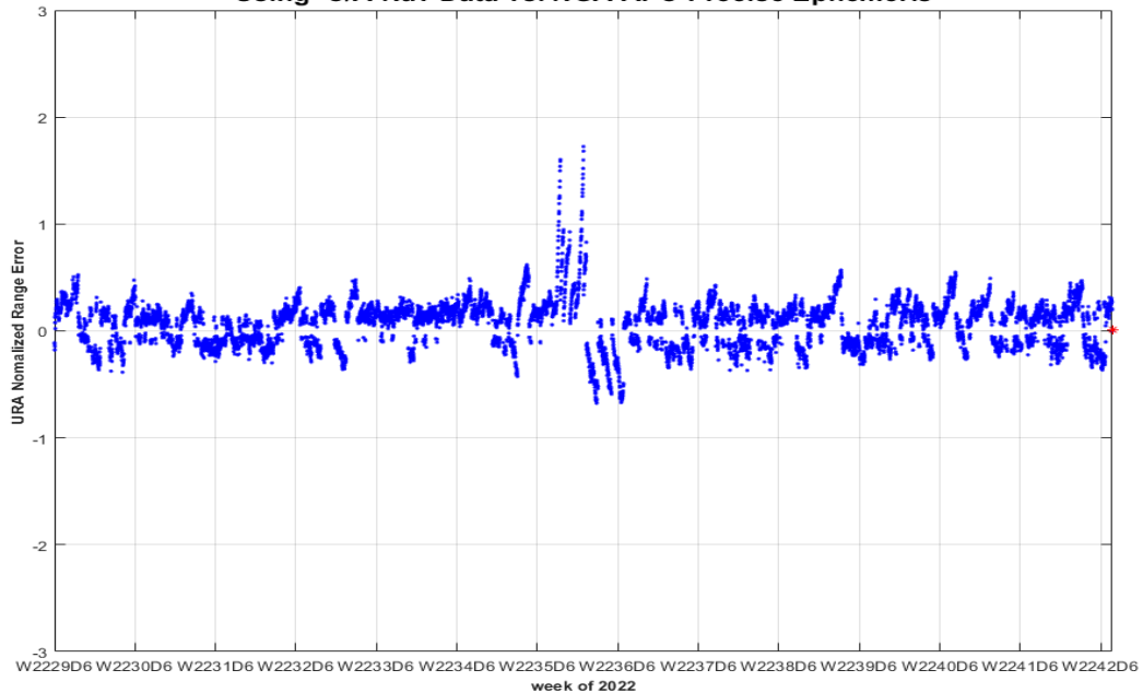
PRN-22 SVN-41 URA Normalized Range Error 10/01/2022 to 12/31/2022 (max in footprint) Using C/A Nav Data vs. NGA APC Precise Ephemeris
