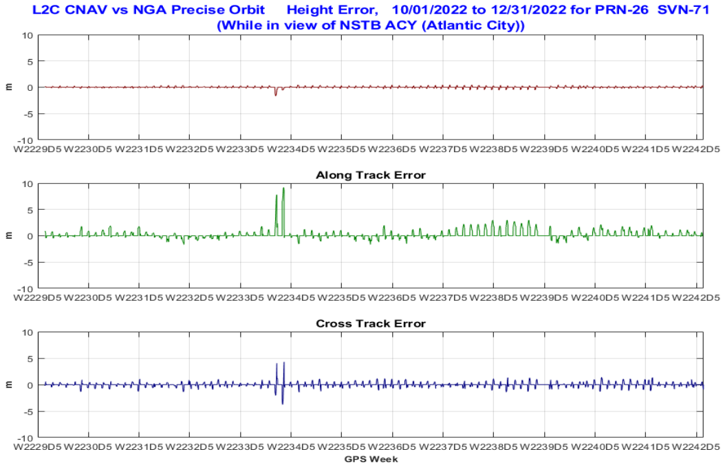
Figure 10-53 Orbit Error PRN26 (SVN71) Using L2C CNAV Data
