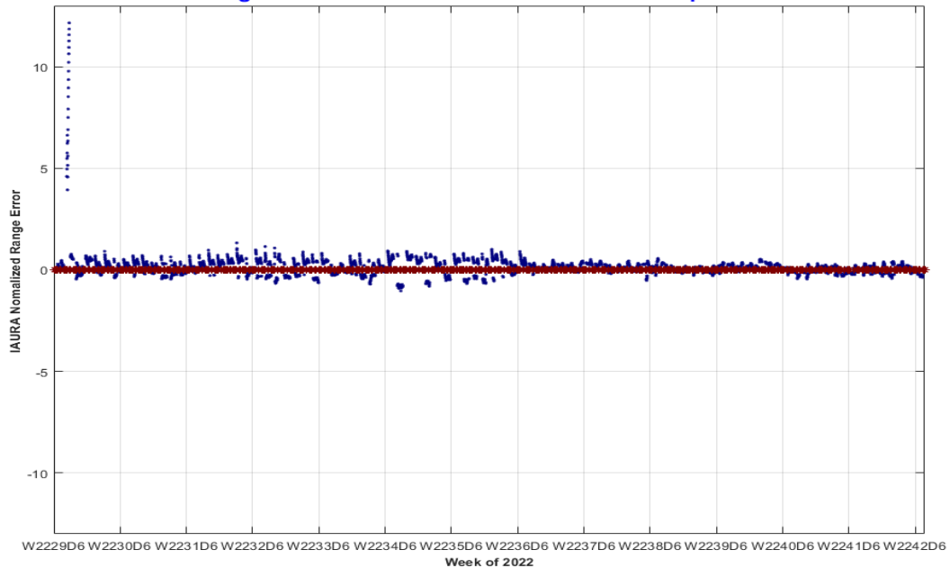
PRN-12 SVN-58 IAURA Normalized Range Error 10/01/2022 to 12/31/2022 (max in footprint) Using L2C CNAV Data vs. NGA APC Precise Ephemeris
