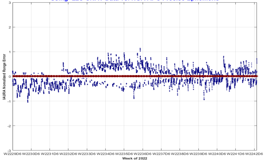
PRN-27 SVN-66 IAURA Normalized Range Error 10/01/2022 to 12/31/2022 (max in footprint) Using L2C CNAV Data vs. NGA APC Precise Ephemeris
