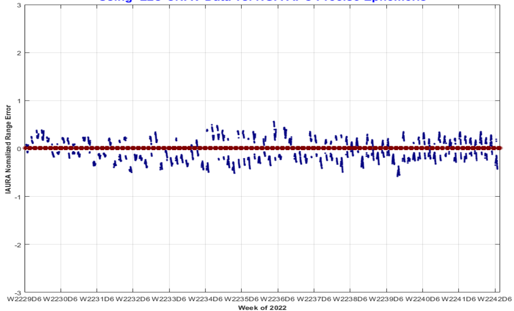
PRN-11 SVN-78 IAURA Normalized Range Error 10/01/2022 to 12/31/2022 (max in footprint) Using L2C CNAV Data vs. NGA APC Precise Ephemeris
