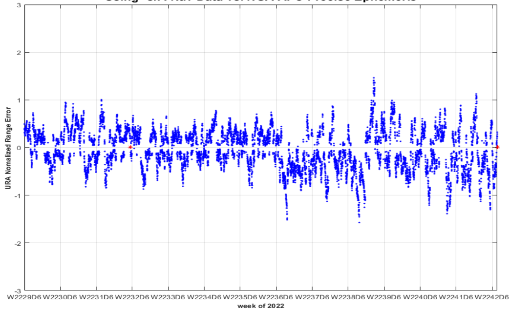
PRN-10 SVN-73 URA Normalized Range Error 10/01/2022 to 12/31/2022 (max in footprint) Using C/A Nav Data vs. NGA APC Precise Ephemeris
