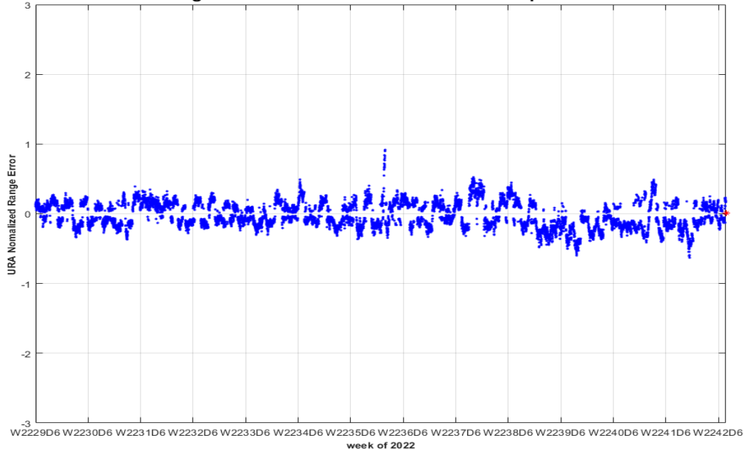
PRN-20 SVN-51 URA Normalized Range Error 10/01/2022 to 12/31/2022 (max in footprint) Using C/A Nav Data vs. NGA APC Precise Ephemeris
