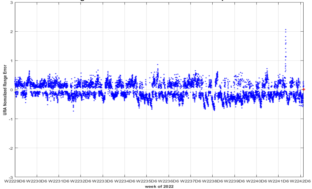
PRN-21 SVN-45 URA Normalized Range Error 10/01/2022 to 12/31/2022 (max in footprint) Using C/A Nav Data vs. NGA APC Precise Ephemeris
