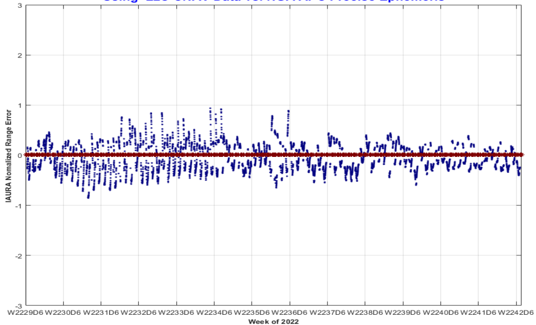
PRN-24 SVN-65 IAURA Normalized Range Error 10/01/2022 to 12/31/2022 (max in footprint) Using L2C CNAV Data vs. NGA APC Precise Ephemeris
