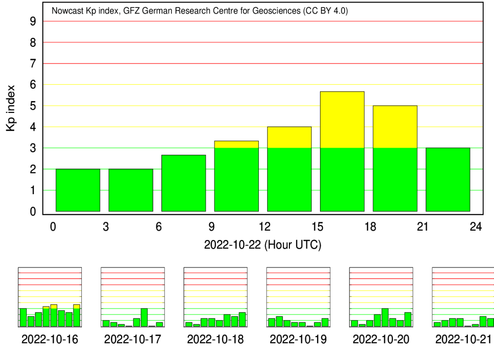
Figure 6-1 K-Index for October 22, 2022
