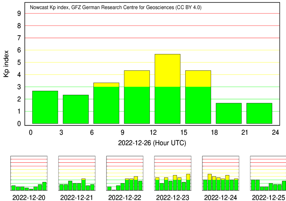
Figure 6-3 K-Index for December 26, 2022
