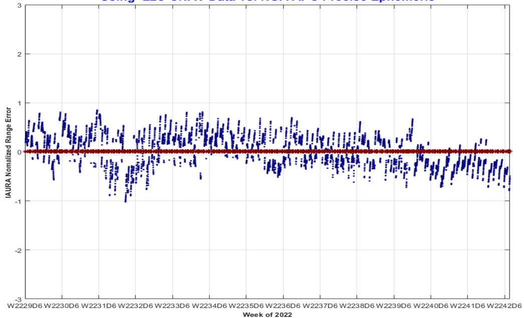
PRN-30 SVN-64 IAURA Normalized Range Error 10/01/2022 to 12/31/2022 (max in footprint) Using L2C CNAV Data vs. NGA APC Precise Ephemeris
