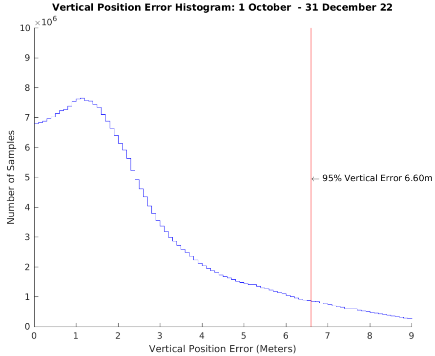
Figure 5-1 Global Vertical Error Histogram
