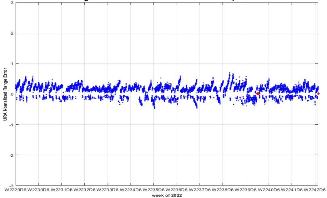
PRN-23 SVN-76 URA Normalized Range Error 10/01/2022 to 12/31/2022 (max in footprint) Using C/A Nav Data vs. NGA APC Precise Ephemeris
