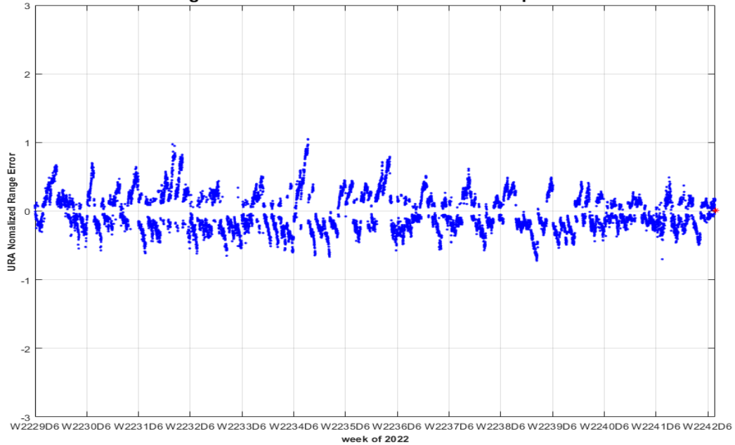
PRN-13 SVN-43 URA Normalized Range Error 10/01/2022 to 12/31/2022 (max in footprint) Using C/A Nav Data vs. NGA APC Precise Ephemeris
