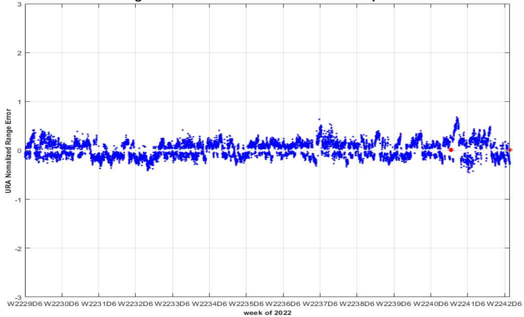
PRN-19 SVN-59 URA Normalized Range Error 10/01/2022 to 12/31/2022 (max in footprint) Using C/A Nav Data vs. NGA APC Precise Ephemeris
