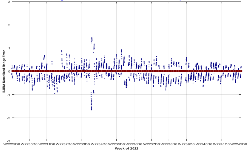
PRN-26 SVN-71 IAURA Normalized Range Error 10/01/2022 to 12/31/2022 (max in footprint) Using L2C CNAV Data vs. NGA APC Precise Ephemeris
