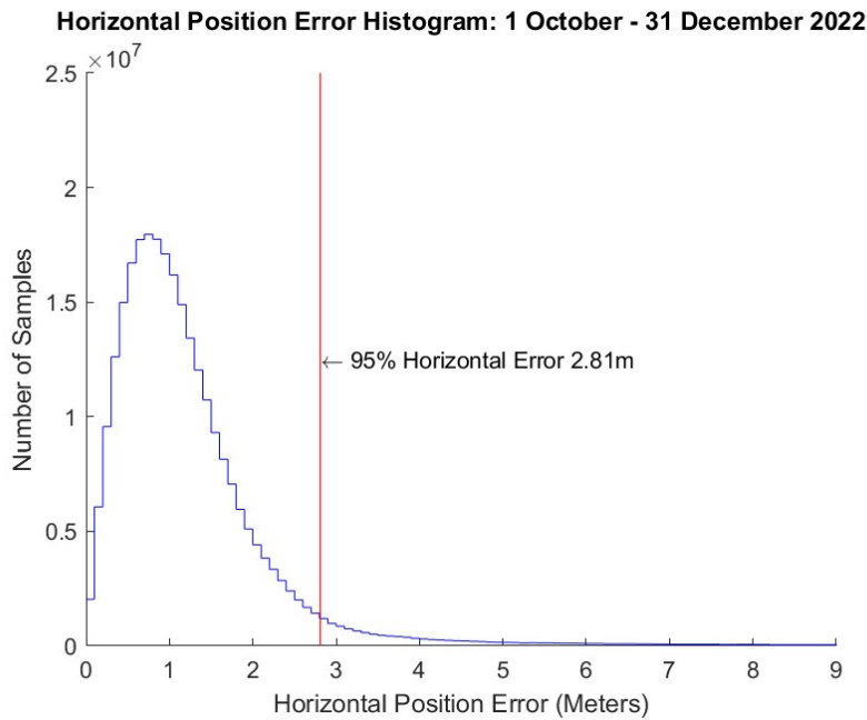
Figure 5-2 Global Horizontal Error Histogram
