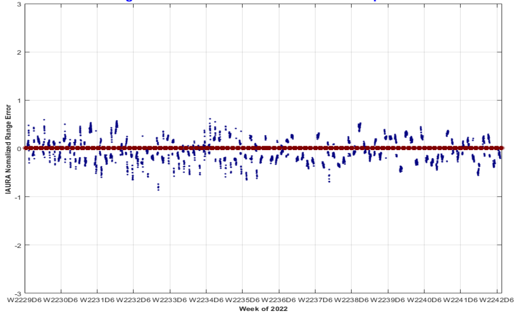
PRN-15 SVN-55 IAURA Normalized Range Error 10/01/2022 to 12/31/2022 (max in footprint) Using L2C CNAV Data vs. NGA APC Precise Ephemeris
