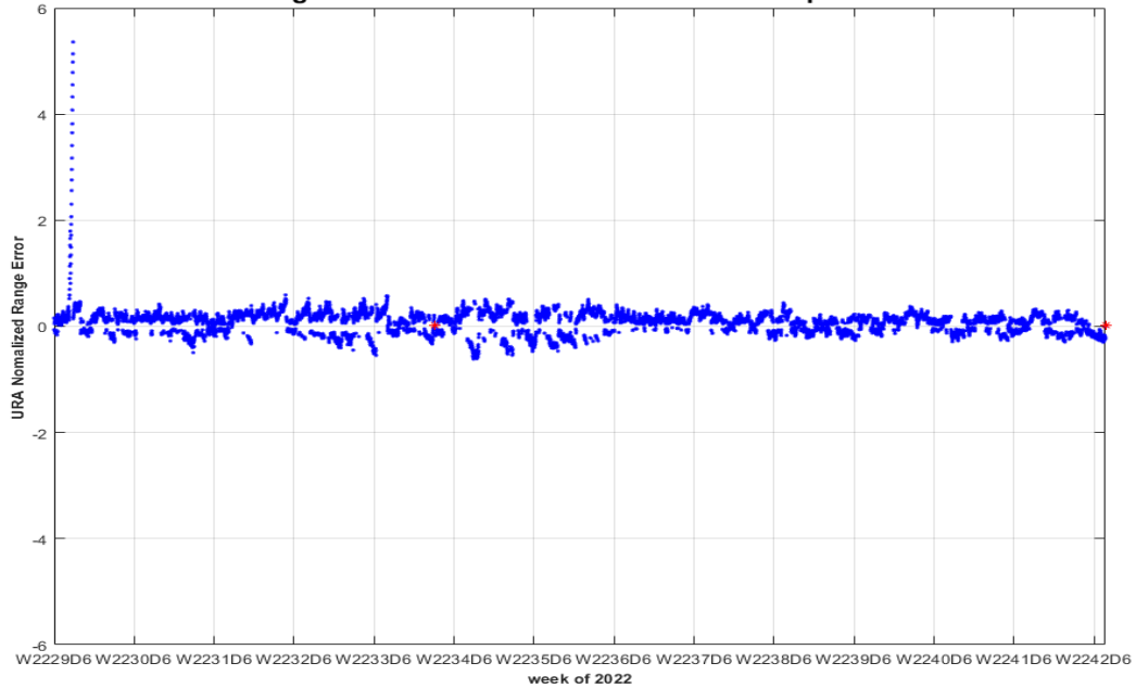
PRN-12 SVN-58 URA Normalized Range Error 10/01/2022 to 12/31/2022 (max in footprint) Using C/A Nav Data vs. NGA APC Precise Ephemeris
