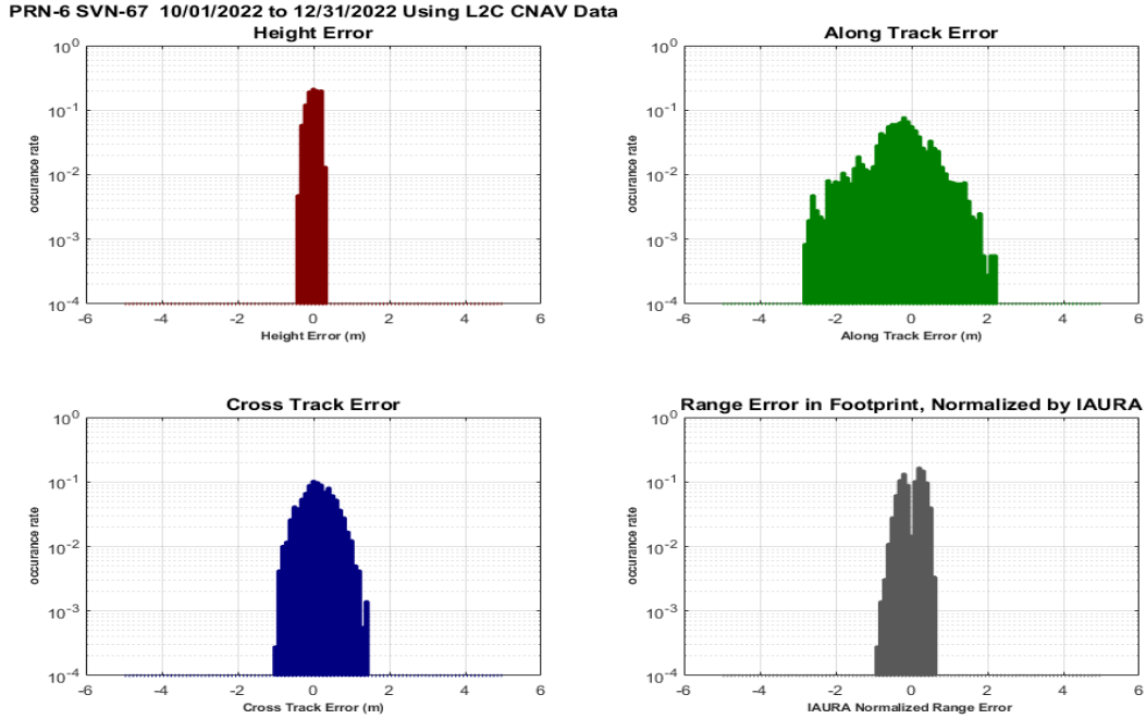
Figure 10-89 Histograms of H, A, C, and Range Error PRN6 (SVN67) Using L2C CNAV Data
