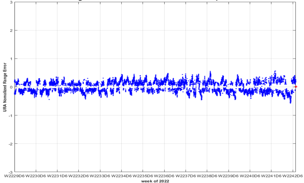
PRN-16 SVN-56 URA Normalized Range Error 10/01/2022 to 12/31/2022 (max in footprint) Using C/A Nav Data vs. NGA APC Precise Ephemeris
