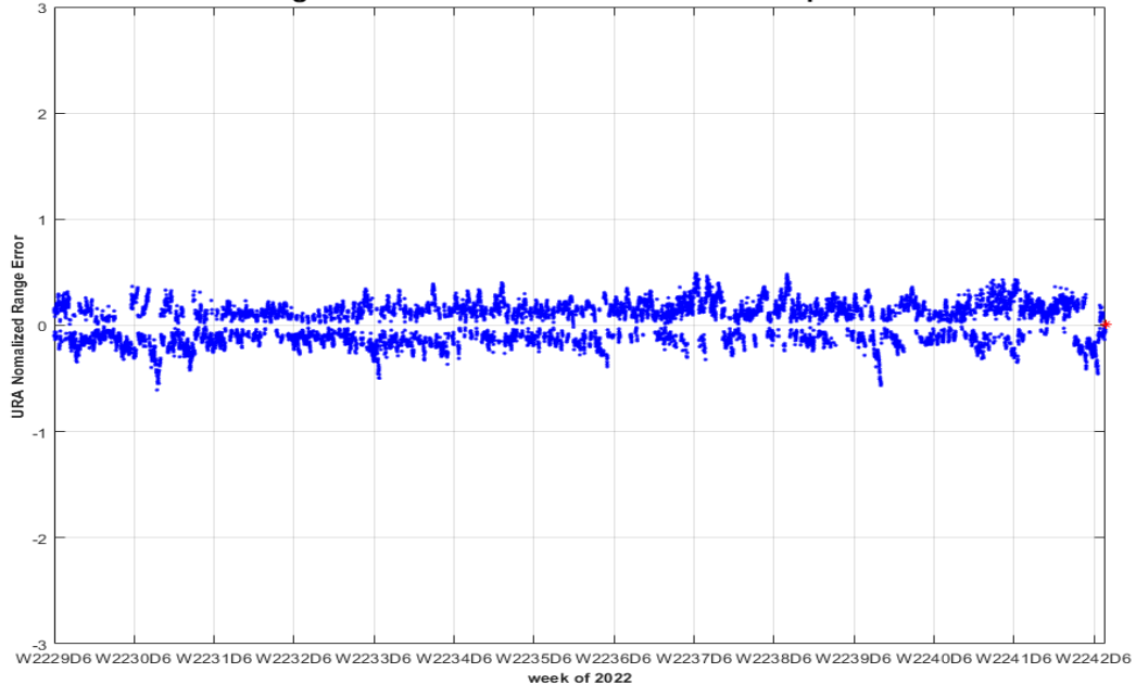
PRN-14 SVN-77 URA Normalized Range Error 10/01/2022 to 12/31/2022 (max in footprint) Using C/A Nav Data vs. NGA APC Precise Ephemeris
